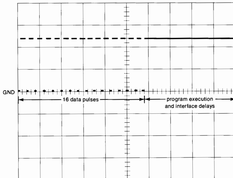
Illustration of Repeat Mode and Delay Before Next Cycle
